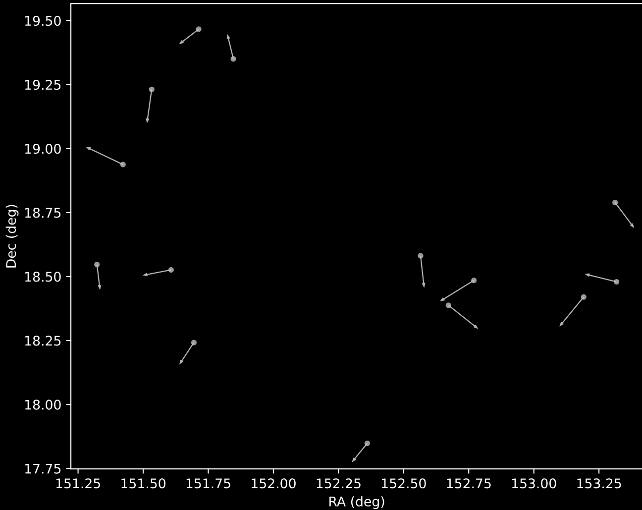
GALAH DR4 Cluster 15 Proper Motion Vectors (n=14)
