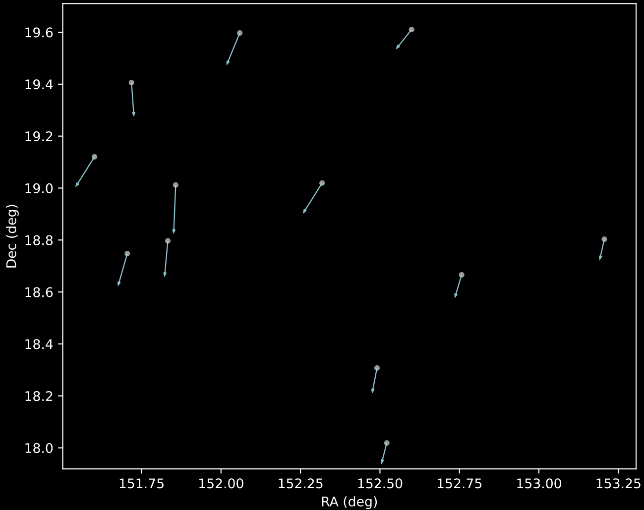
GALAH DR4 Cluster 19 Proper Motion Vectors (n=12)
