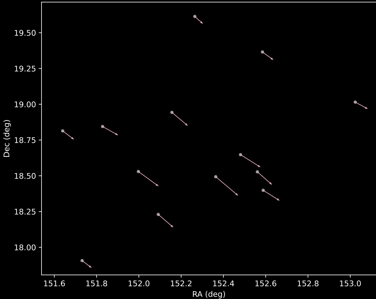
GALAH DR4 Cluster 13 Proper Motion Vectors (n=13)
