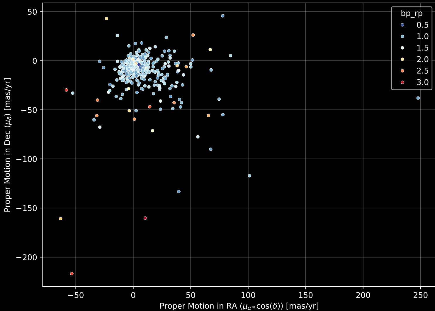
GALAH DR4 Field: [6602] Proper Motion Diagram (n= 453)
