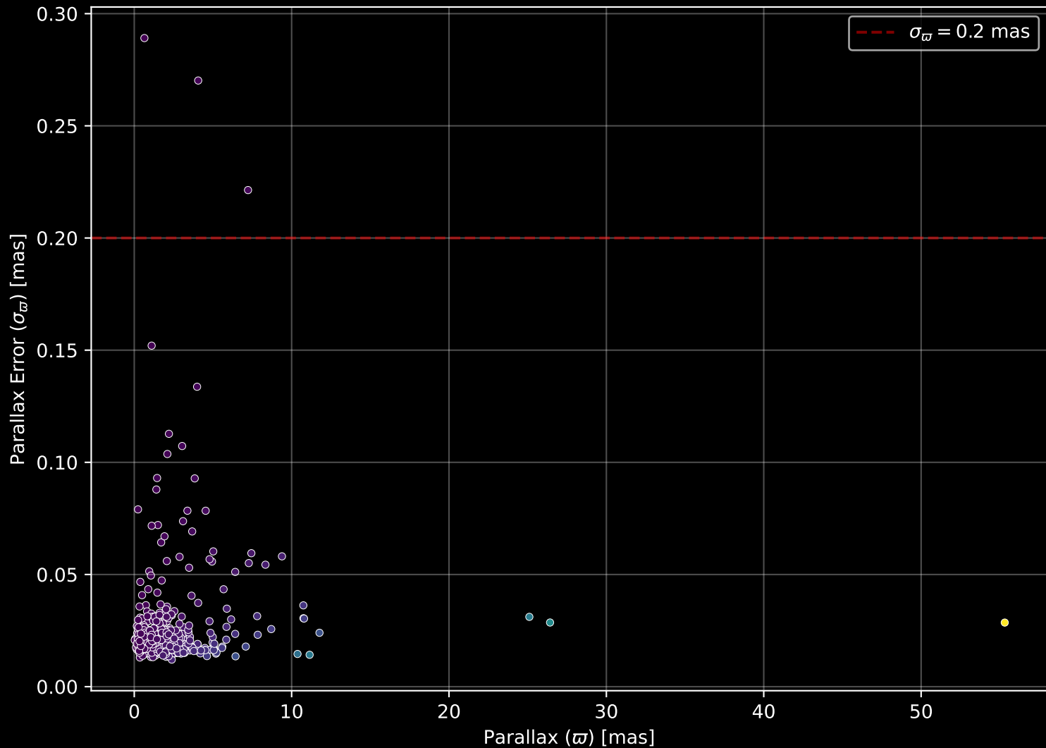
GALAH DR4 Field: [6602] Parallax Quality (n= 453)
