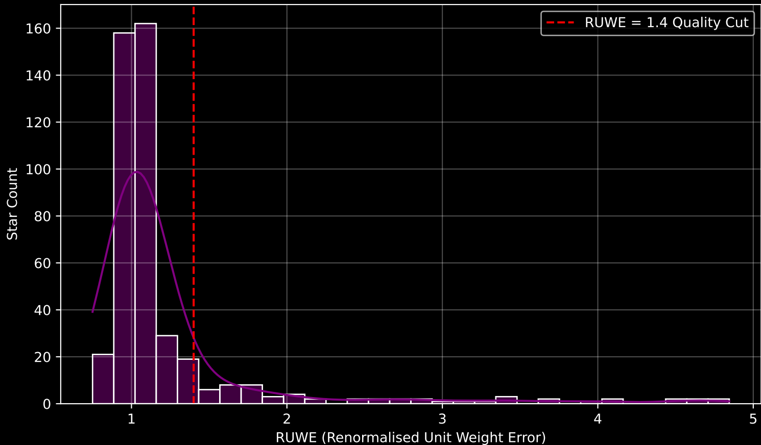
GALAH DR4 Field [6602] RUWE Distribution (n= 445)
