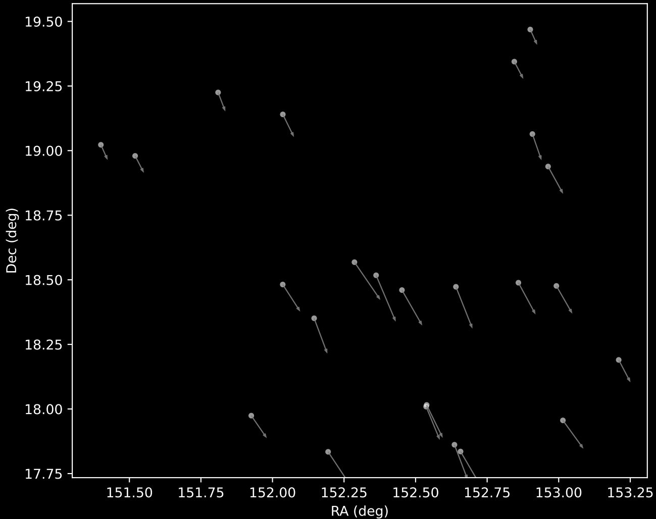
GALAH DR4 Cluster 14 Proper Motion Vectors (n=24)
