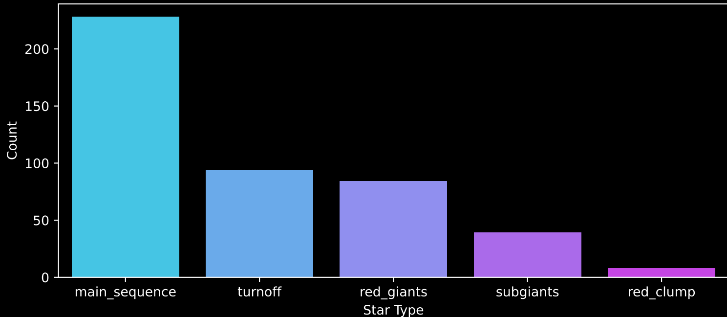
GALAH DR4 Field: [6602] Count plot of Star Type
