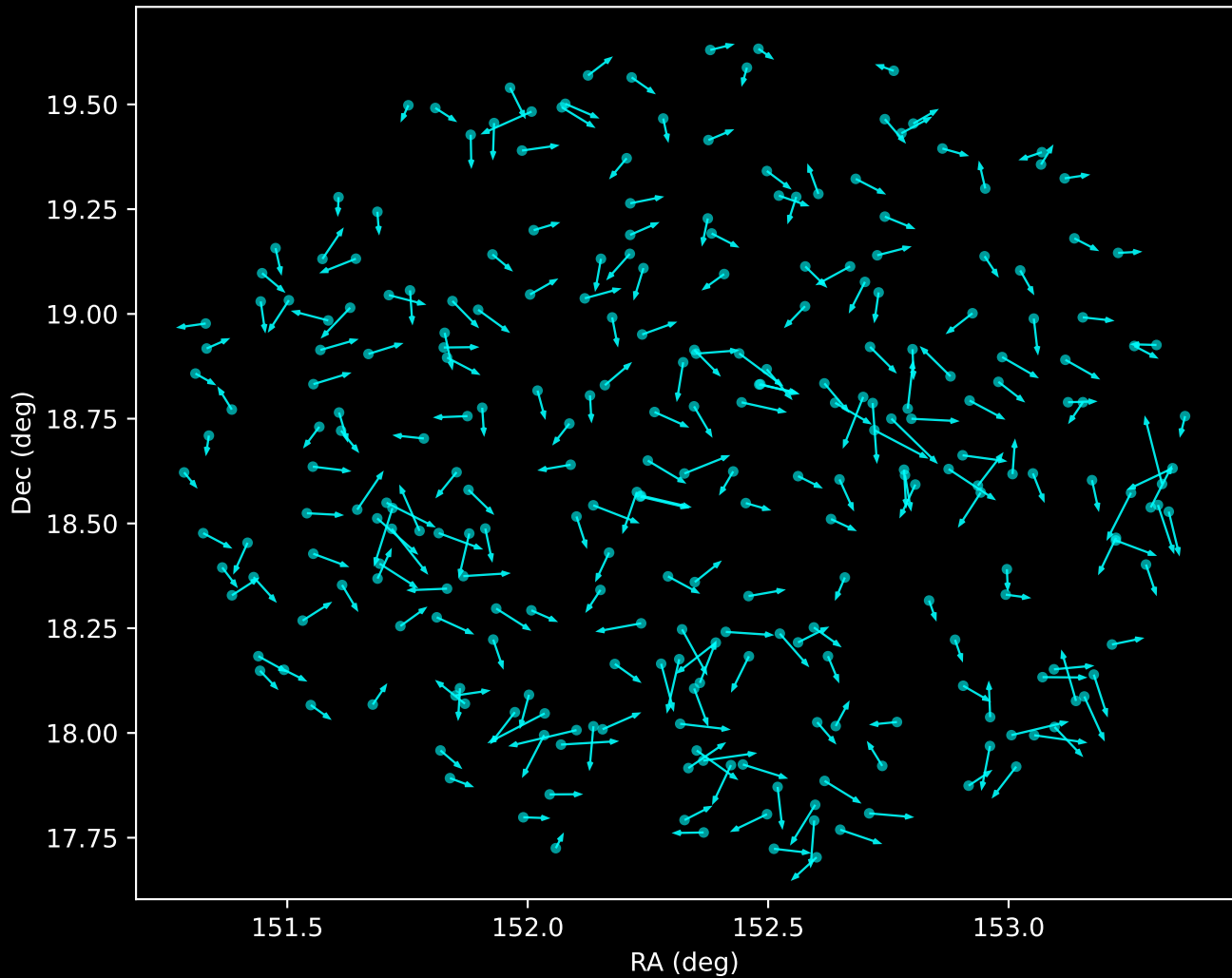
GALAH DR4 Noise Stream Proper Motion Vectors (n=267)
