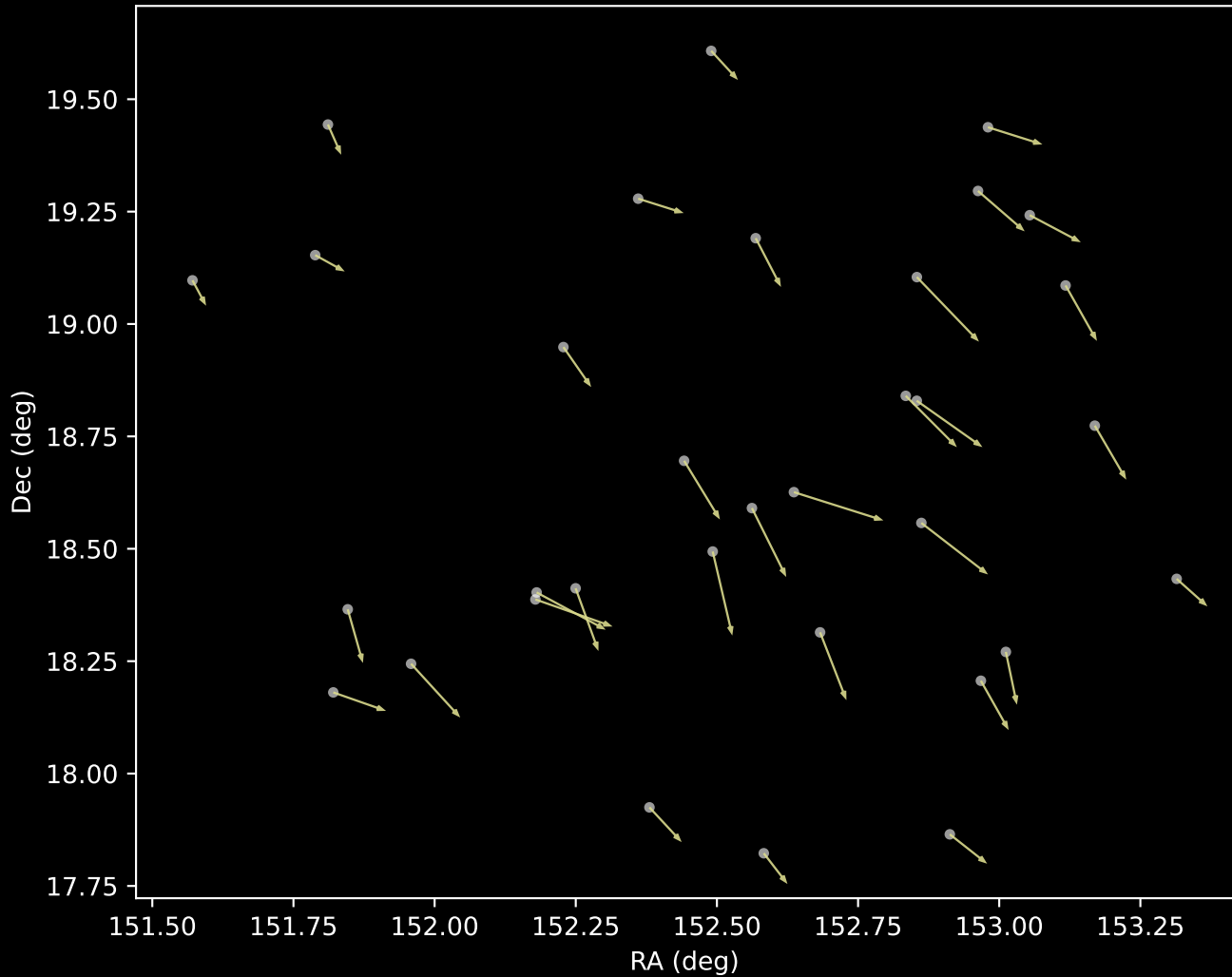
GALAH DR4 Cluster 17 Proper Motion Vectors (n=33)
